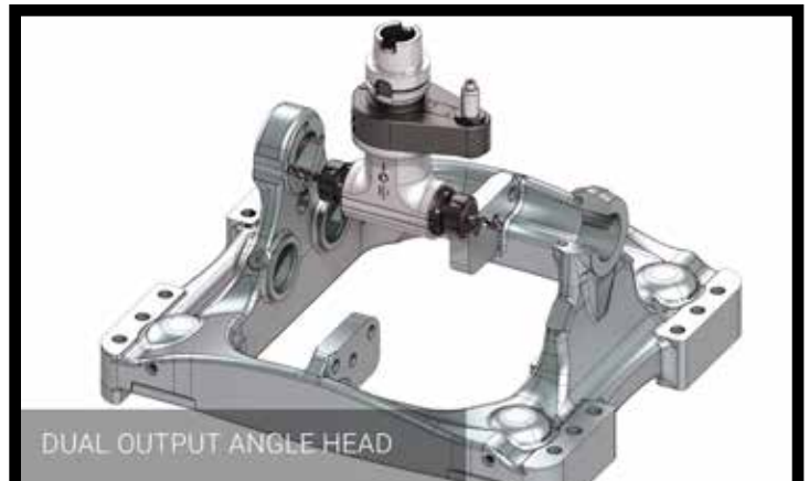
All common tool shanks available e.g. CAT, HSK, CAPTO, KM
