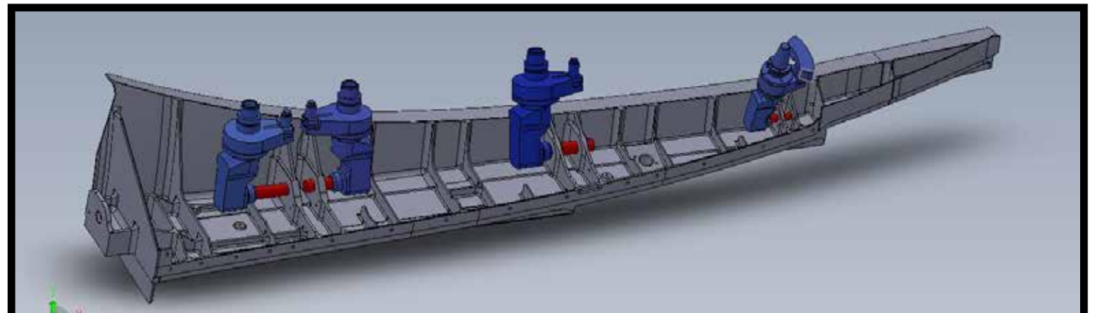
Different outlets from ER-8 to ER-40 as well as CAT40-CAT50 for heavy duty applications
