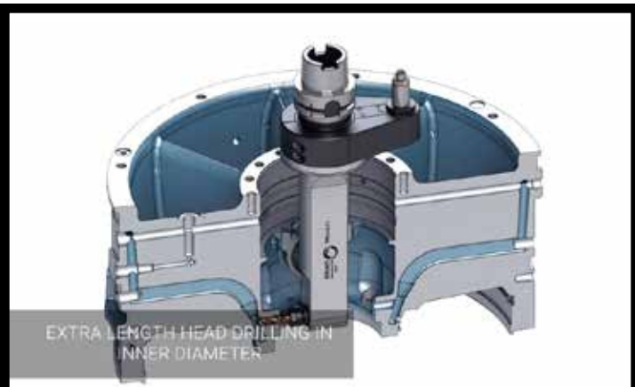
Different styles, length, 90 degree or adjustable heads available.
