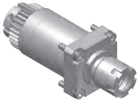
STR161000 Cross drilling/milling unit RATIO 1 : 1 RPM(MAX) 8000 TOOL CLAMPING ER16M
